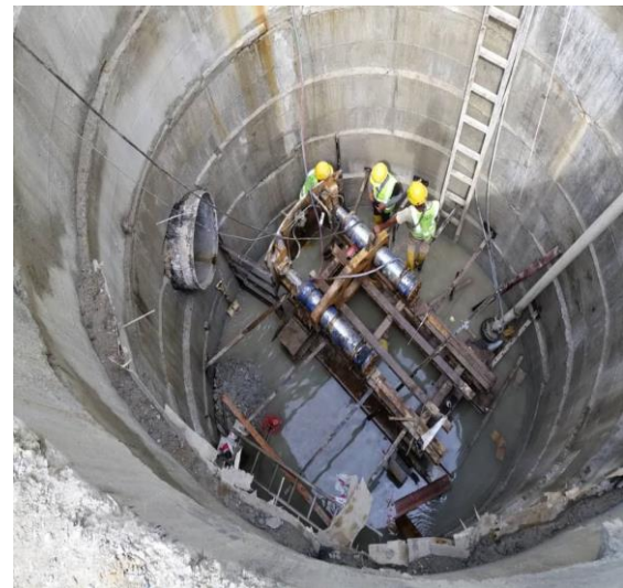
MH5 –MH5S – MH6s – Manshield pipe sleeve jacking
